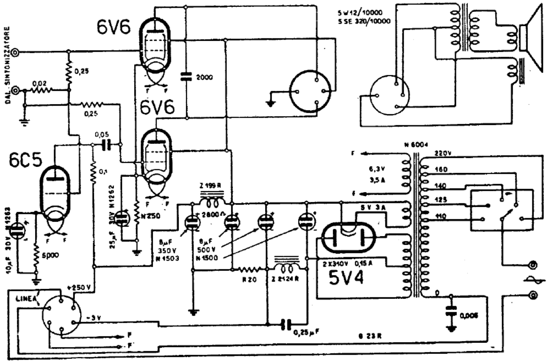
Geloso G23R Power Supply and Amplifier
